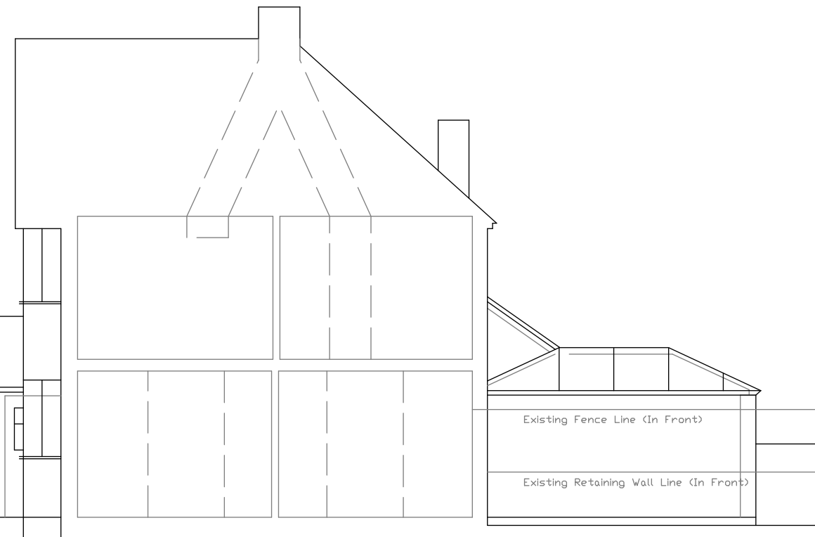
East Elevation (Part Section)
