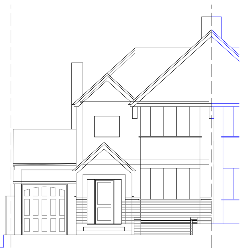
South Elevation (Front)
