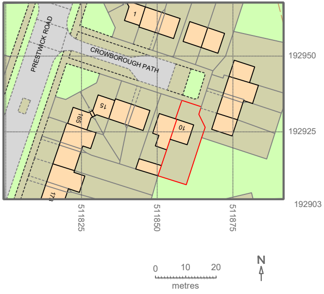
Site plan (1:1250)
