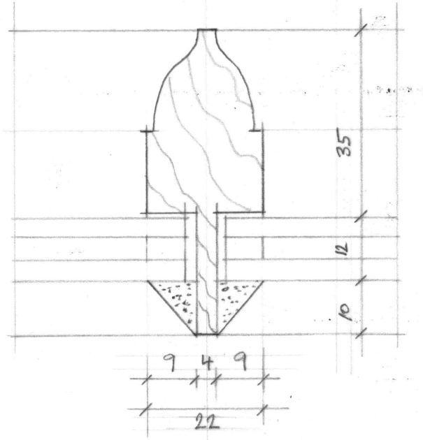
FULL SIZE GLAZING BAR SECTION LAMBS TONGUE OVULO 22 x 57 MM
