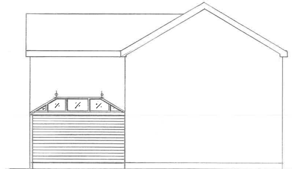
PROPOSED SIDE ELEVATION - N
