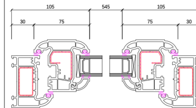
Cross section S2, M 5:1
