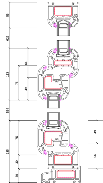
Cross section S2, M 5:1
