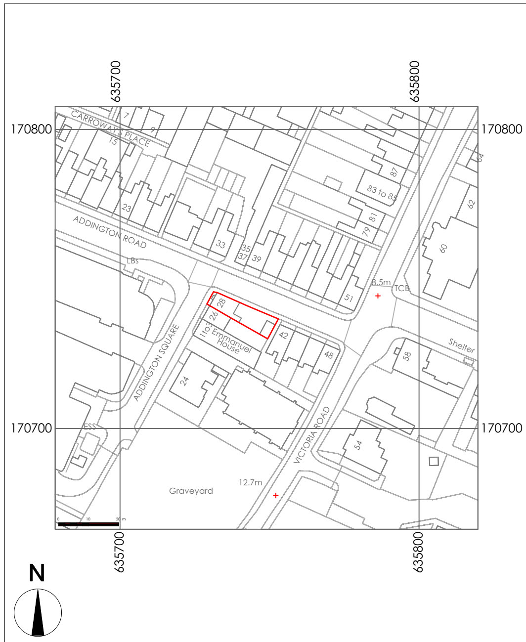
LOCATION PLAN - 1:1250
