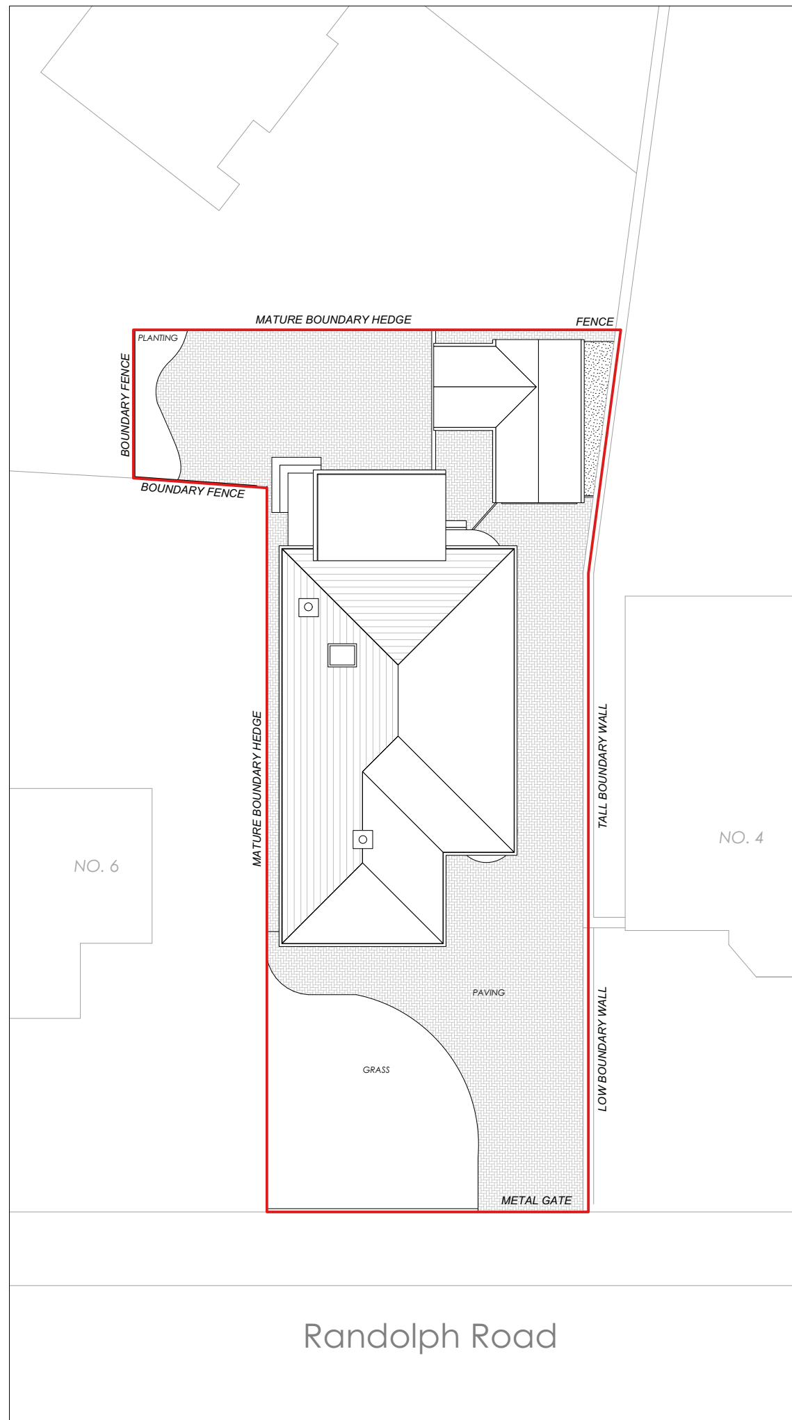
1 Site Plan As Existing (showing roof plan) Scale: 1:200 0 1 2 3 4 5 10m Scale in meters
