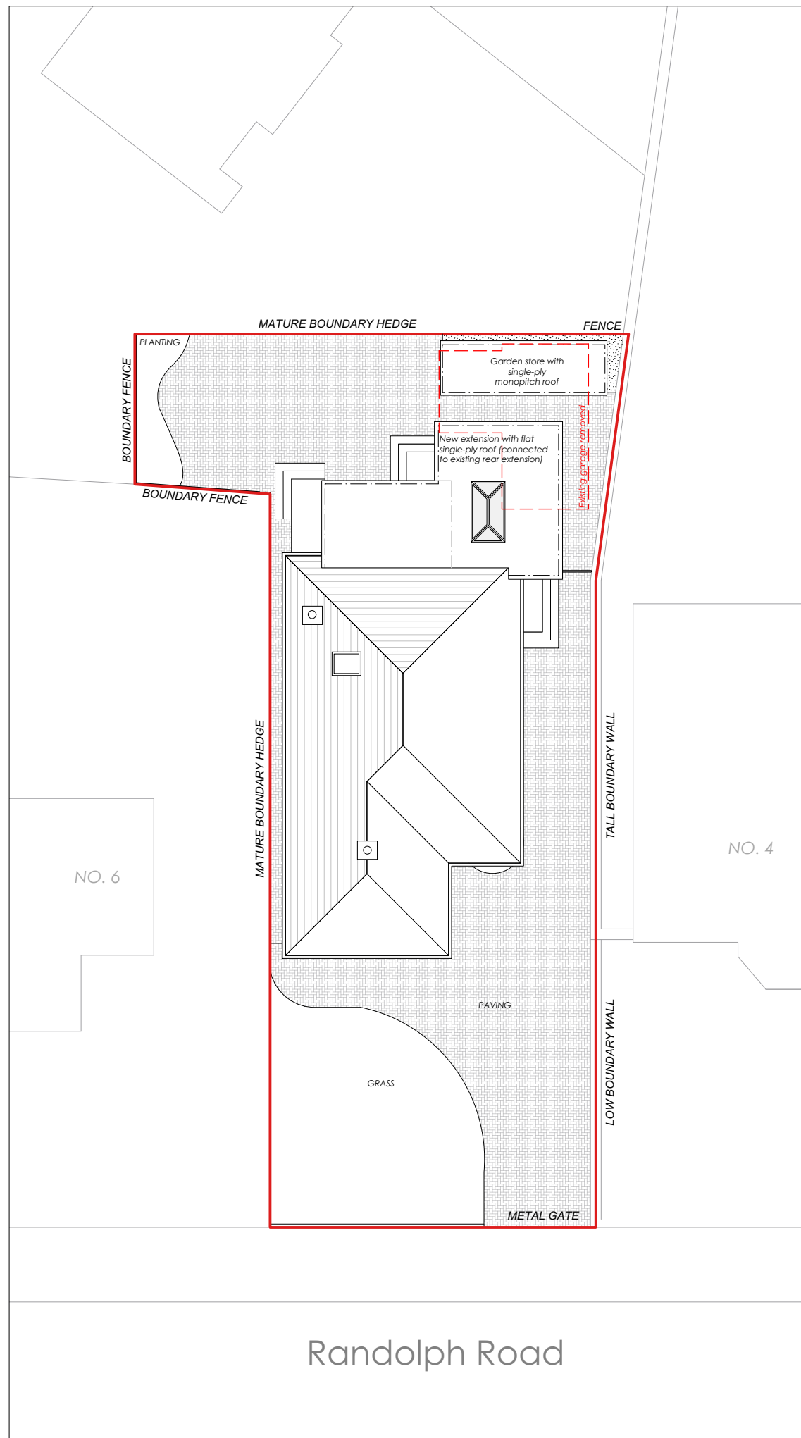
2 Site Plan As Proposed (showing roof plan) Scale: 1:200
