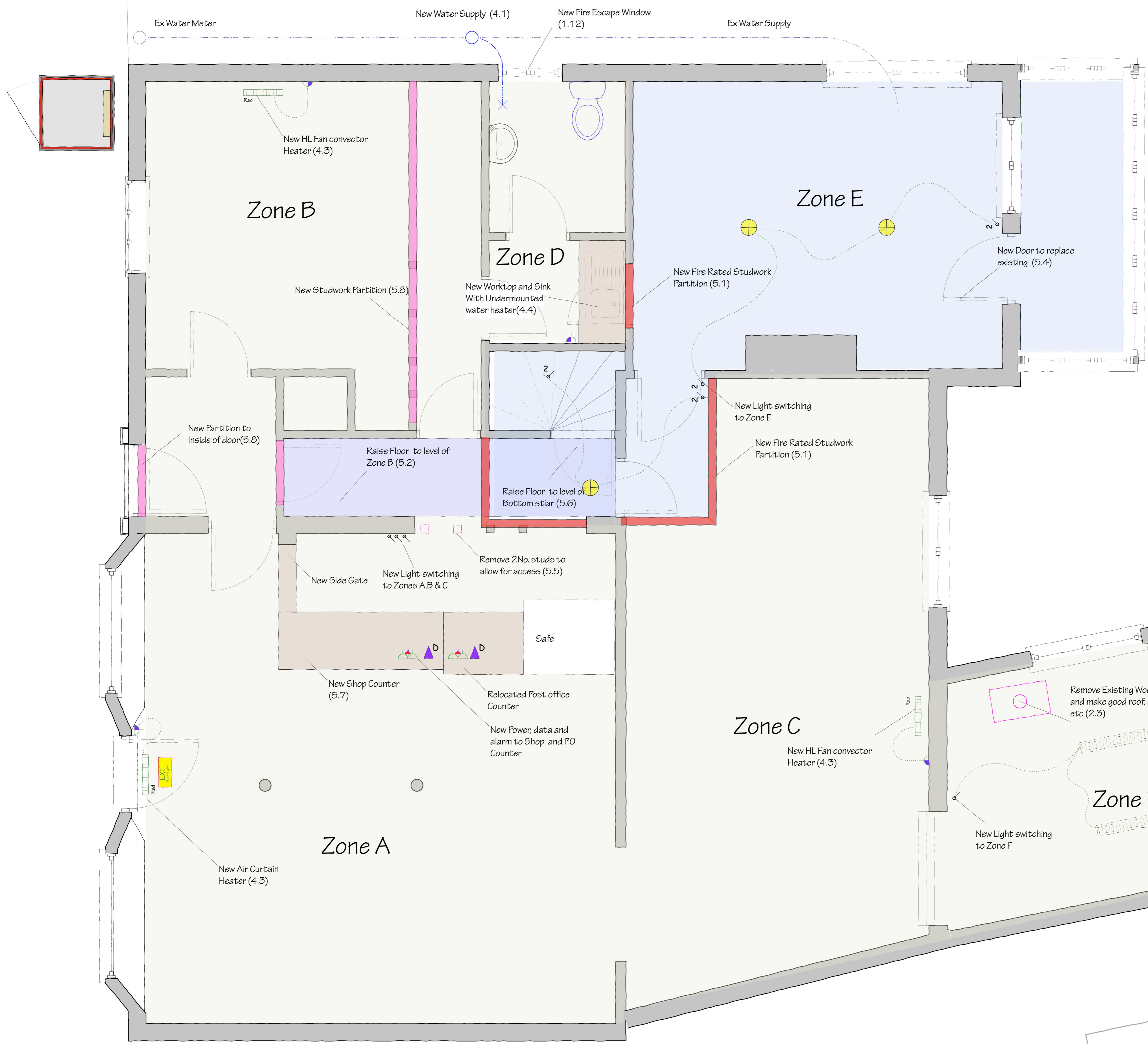
Proposed Ground Floor Plan
