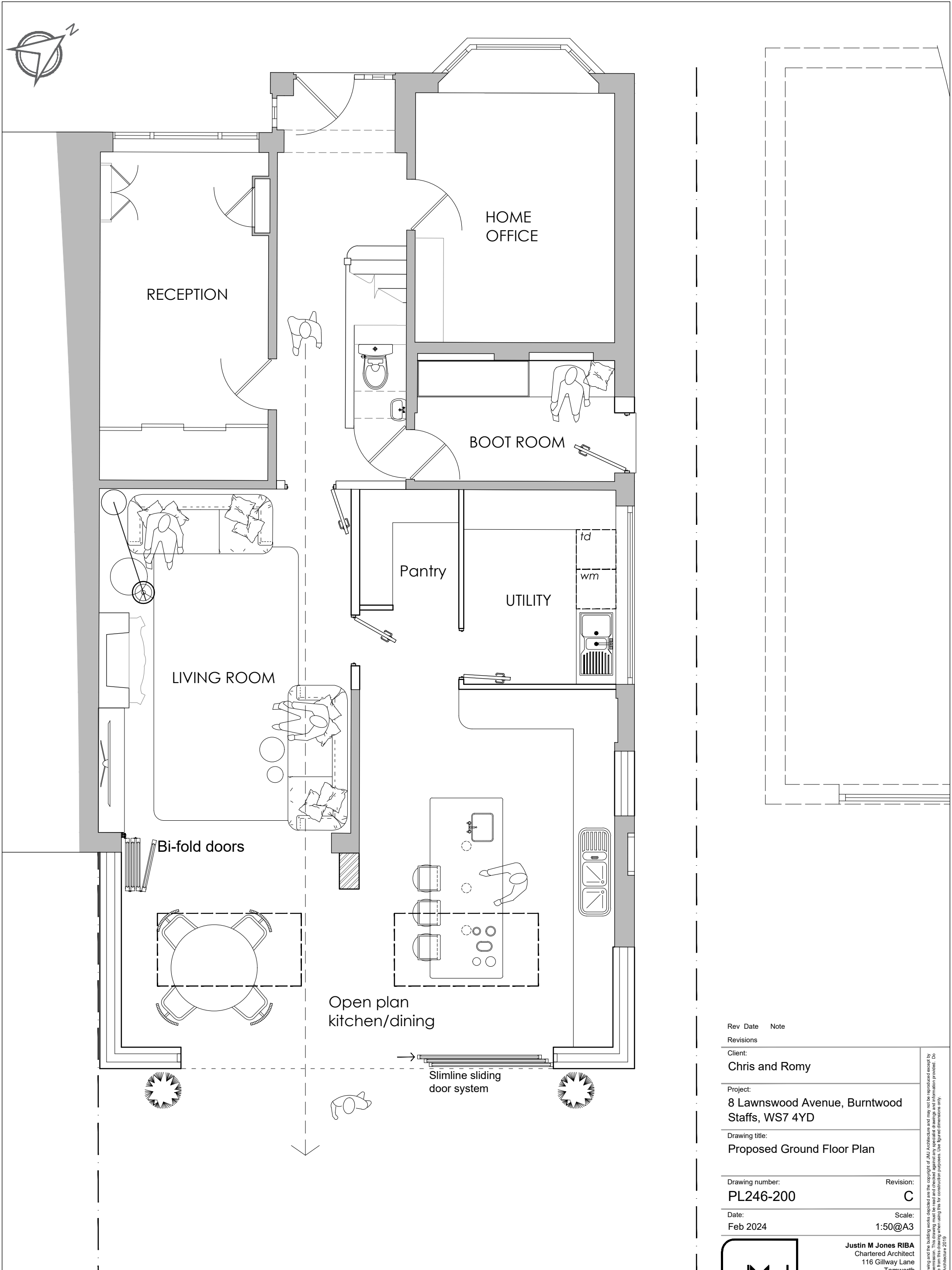
Proposed Ground Floor Plan scale 1:50@A3
