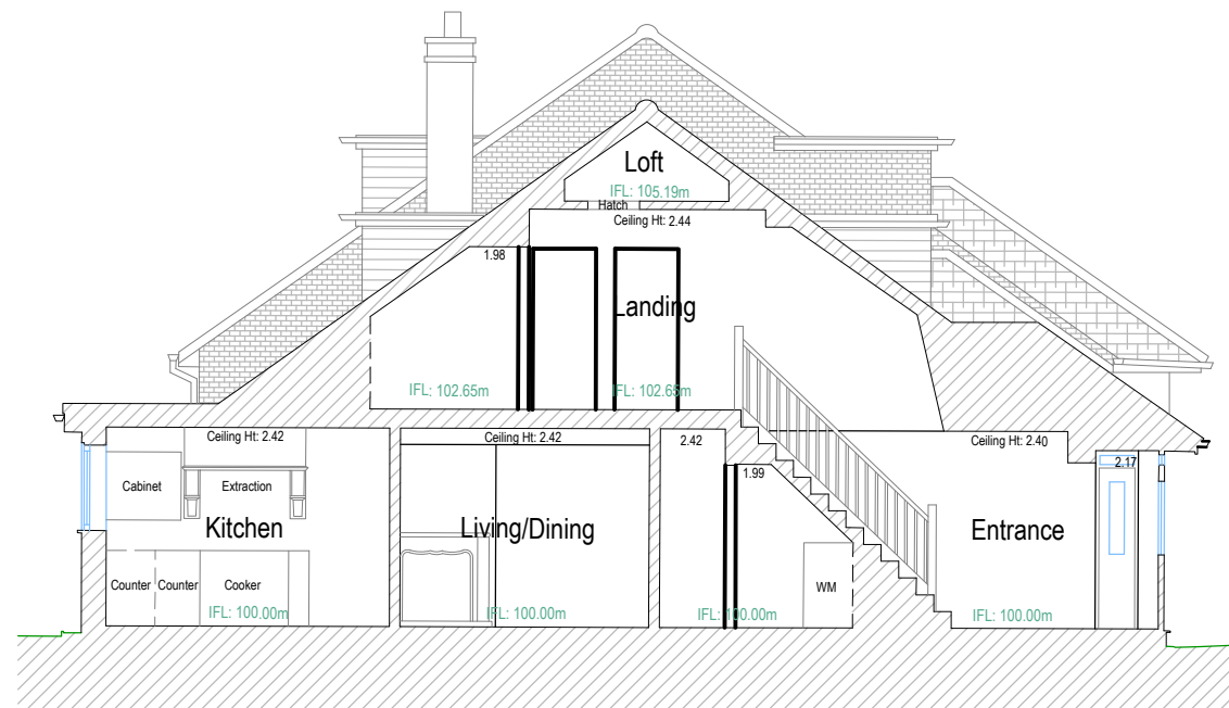
Datum: 98.00m. Section.
