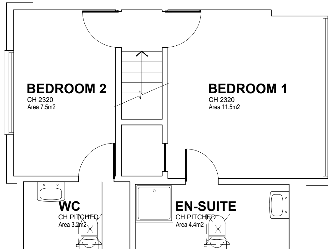
PROPOSED FIRST FLOOR LAYOUT SCALE 1:50
