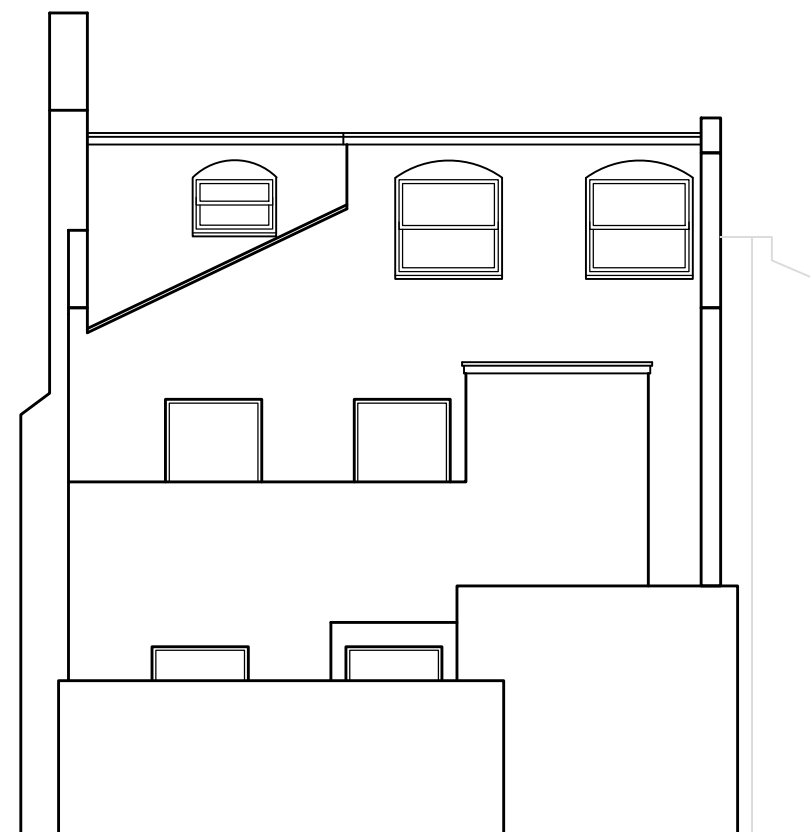
PROPOSED REAR ELEVATIONS
