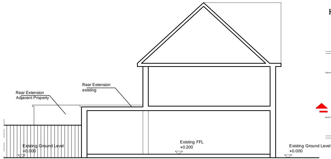
LONG SECTION EXISTING SCALE 1:100
