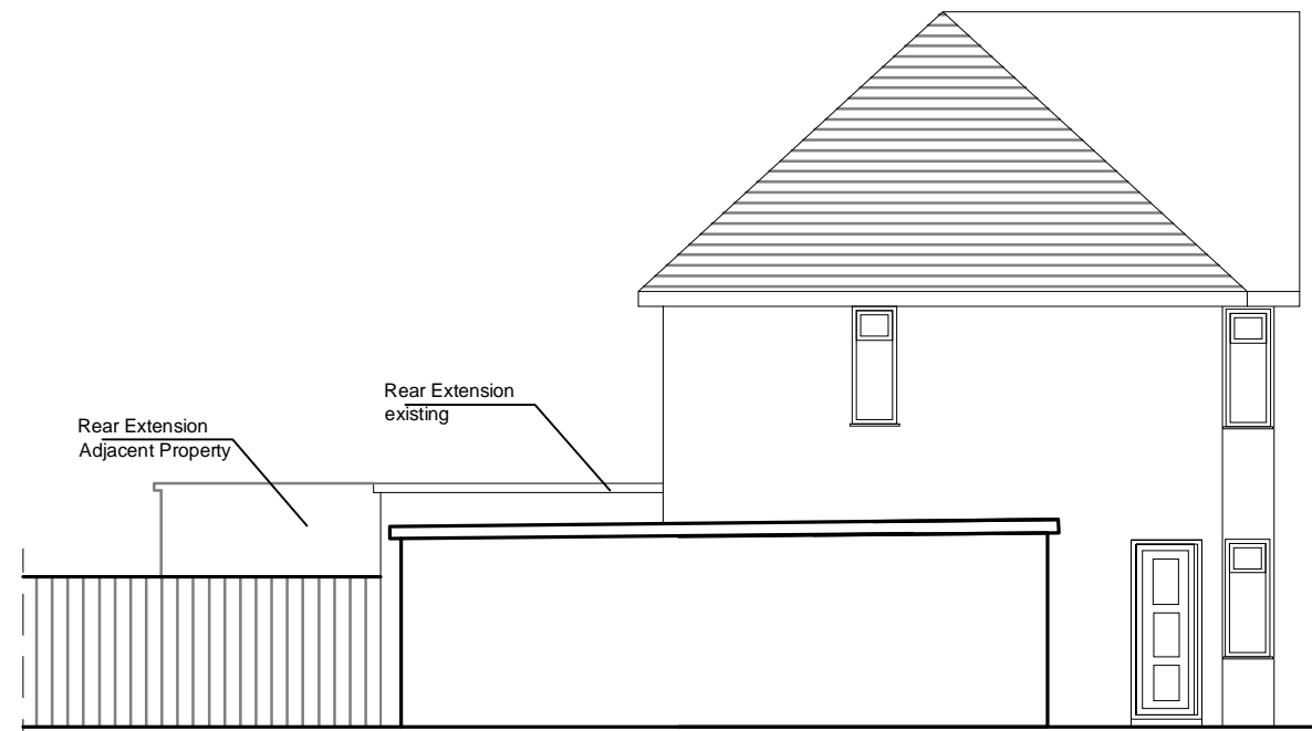
SIDE ELEVATION EXISTING SCALE 1:100
