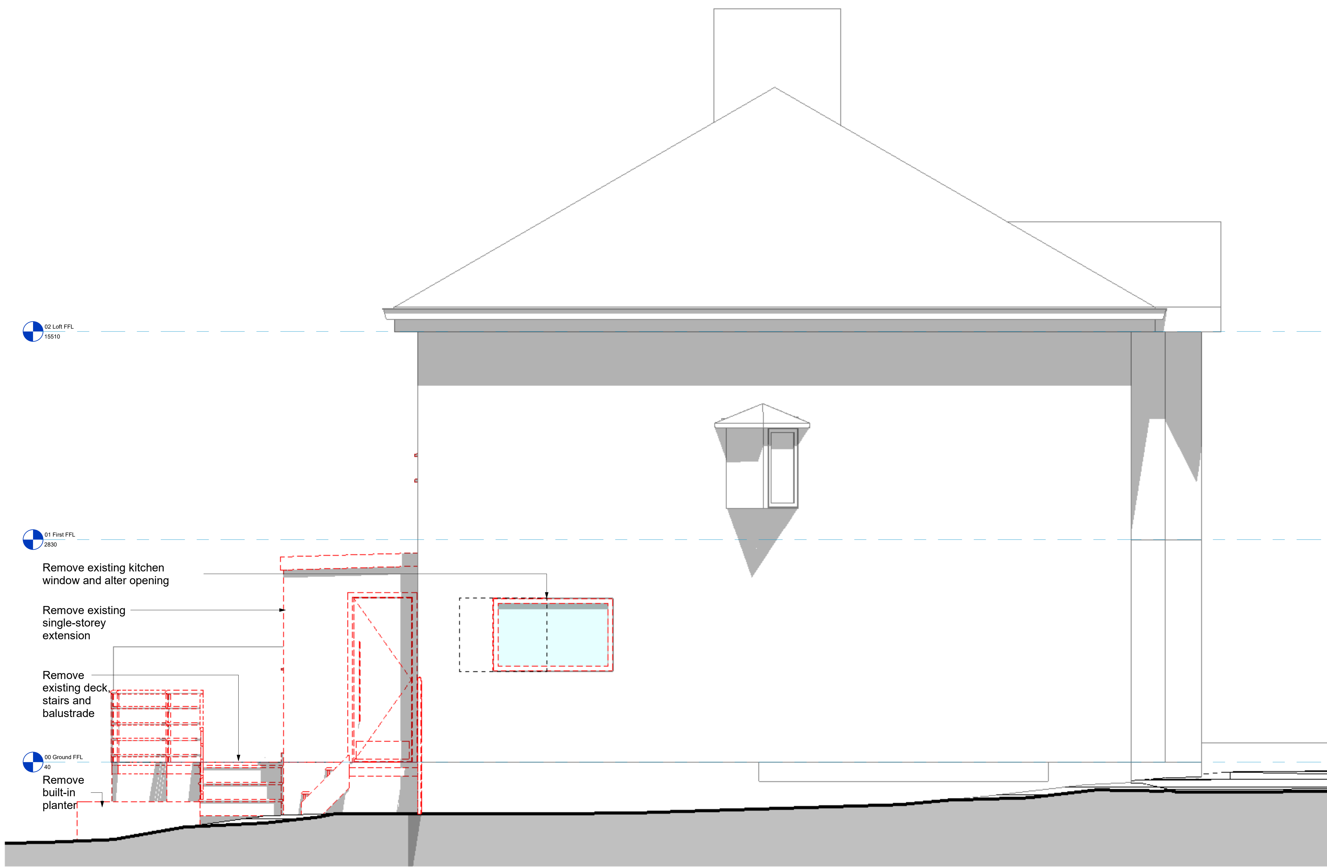
1 South Elevation 1:50 @ A3
