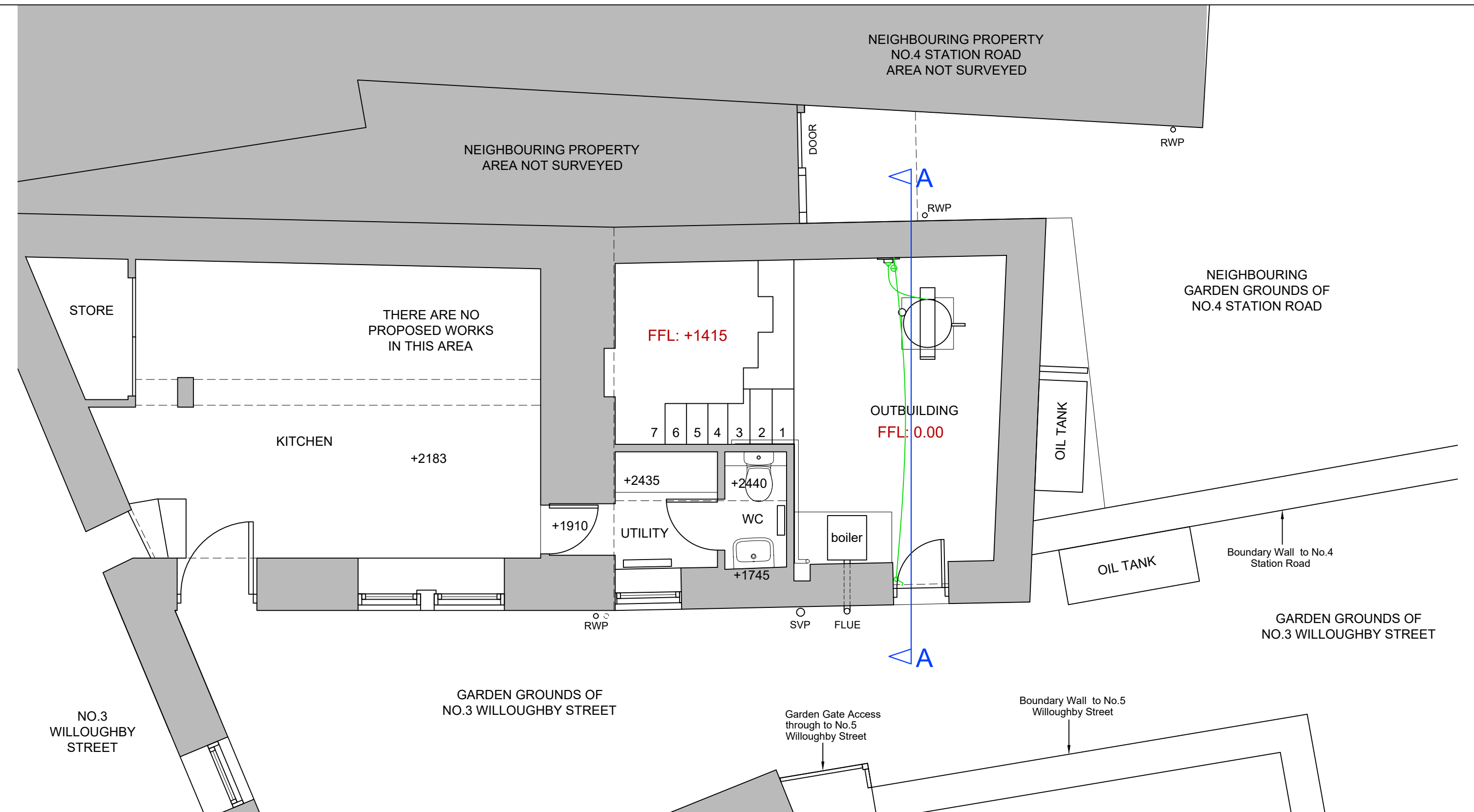
EXISTING GROUND FLOOR PLAN OF OUTBUILDING Scale 1.50
