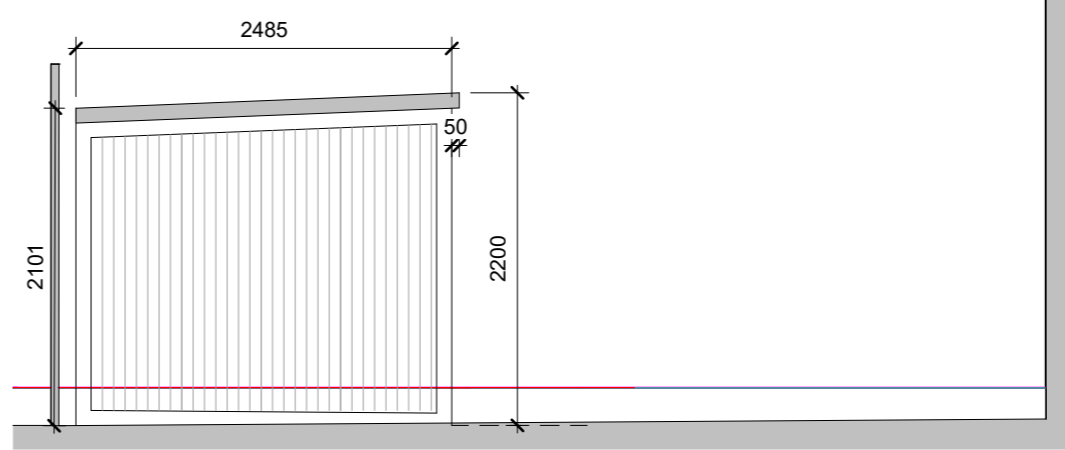
2 Bin Store - North 1 : 50
