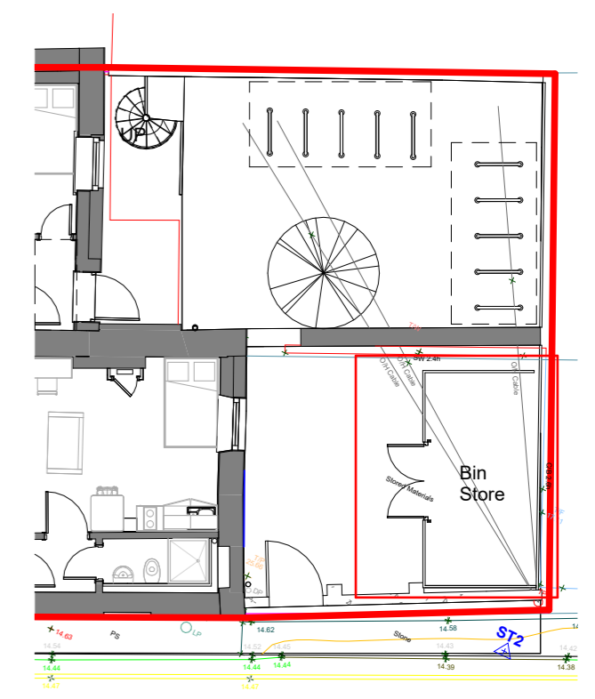
4 Bin Store - Location Plan 1 : 150
