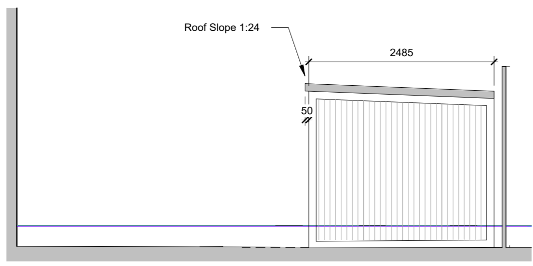
3 Bin Store - South 1 : 50
