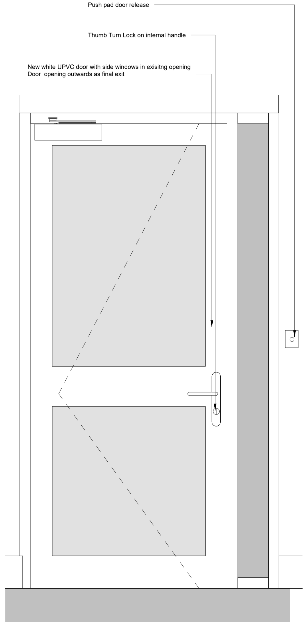
4 ED-0-03 Elevation Internal - LG1 Door East 1 : 10
