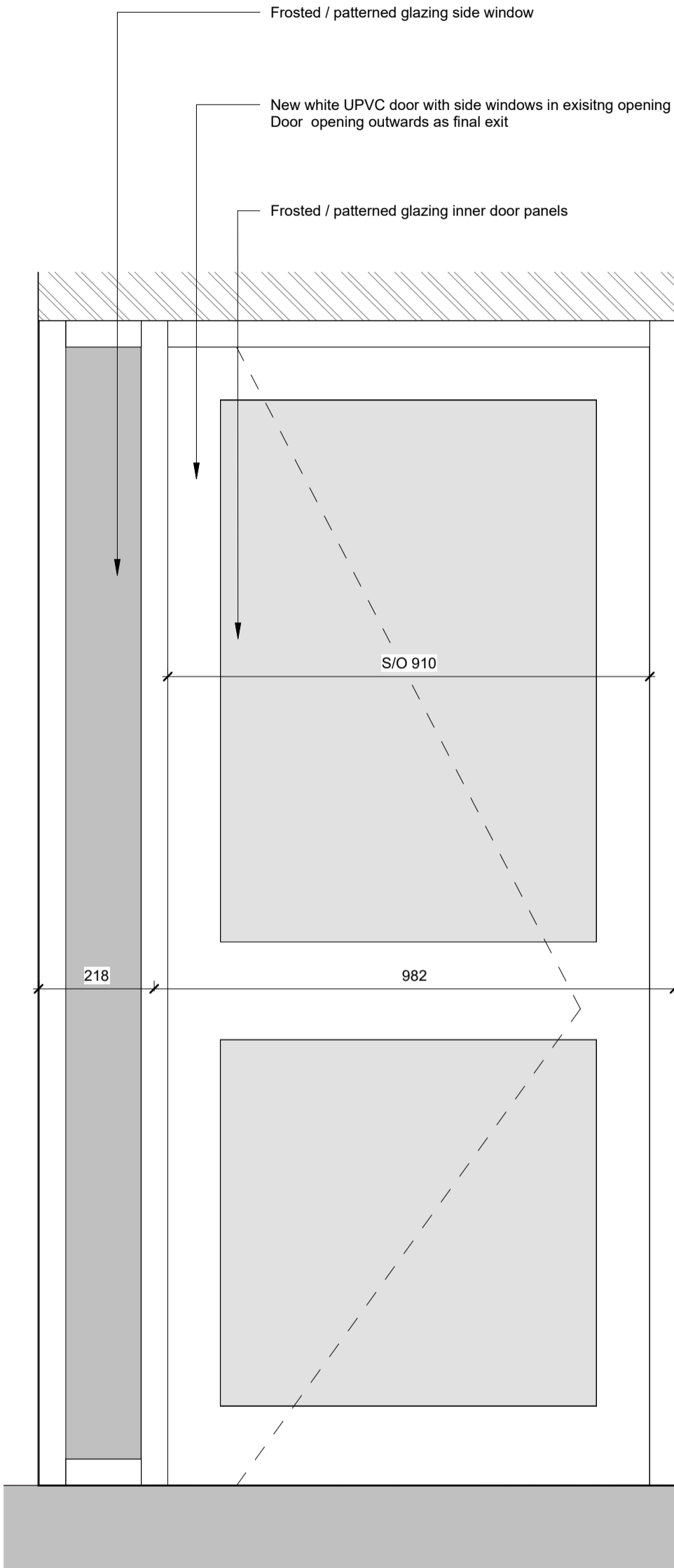
3 ED-0-03 Elevation External - LG1 Door East 1 : 10
