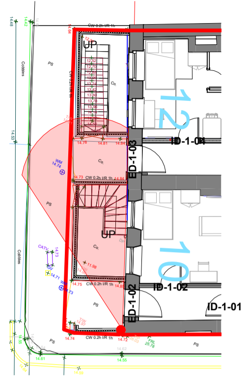
2 Camera 2 Location Plan 1 : 150
