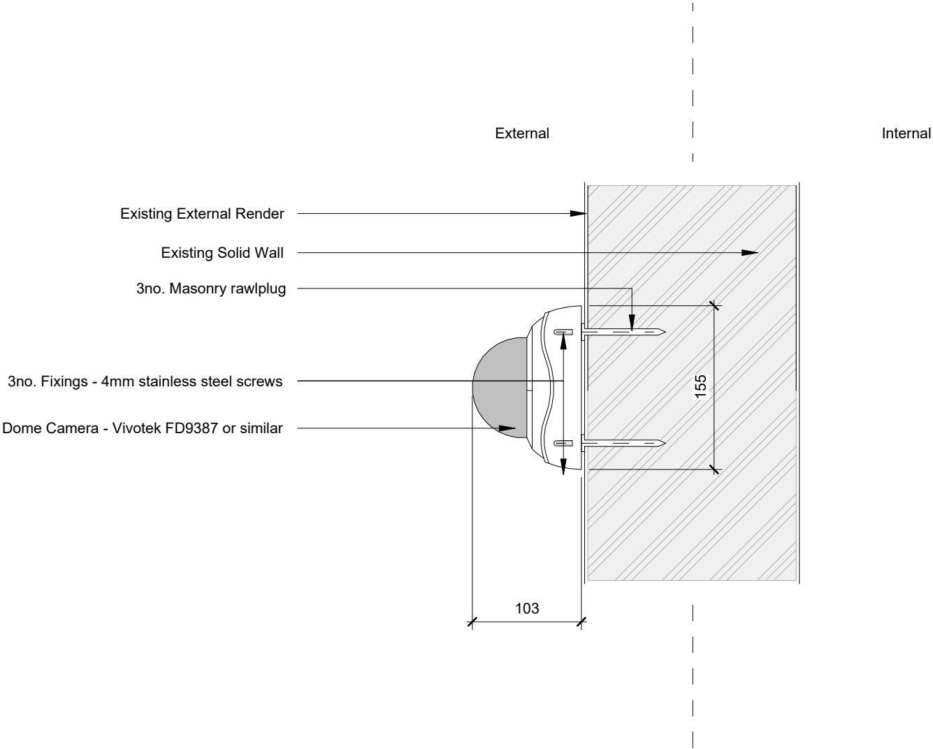
1 Dome camera fixing detail 1 : 5
