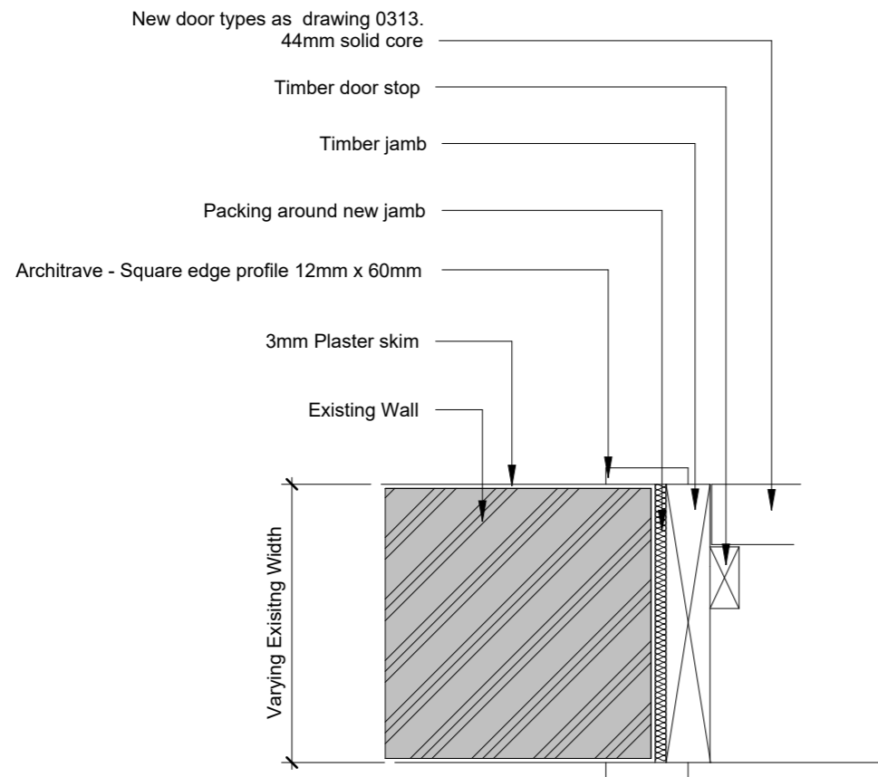
1 Typical Internal Door Jamb 1 : 5
