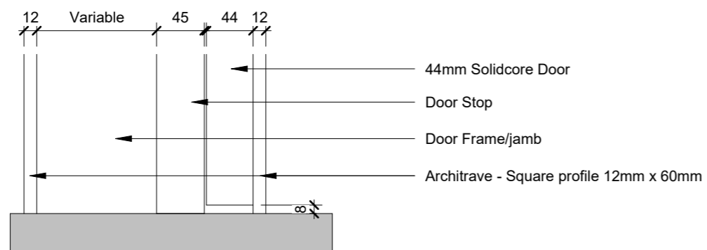
3 Typical Internal Door Cill 1 : 5
