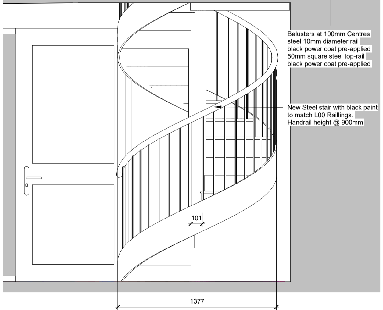
1 Proposed Stair Elevation 1 : 20
