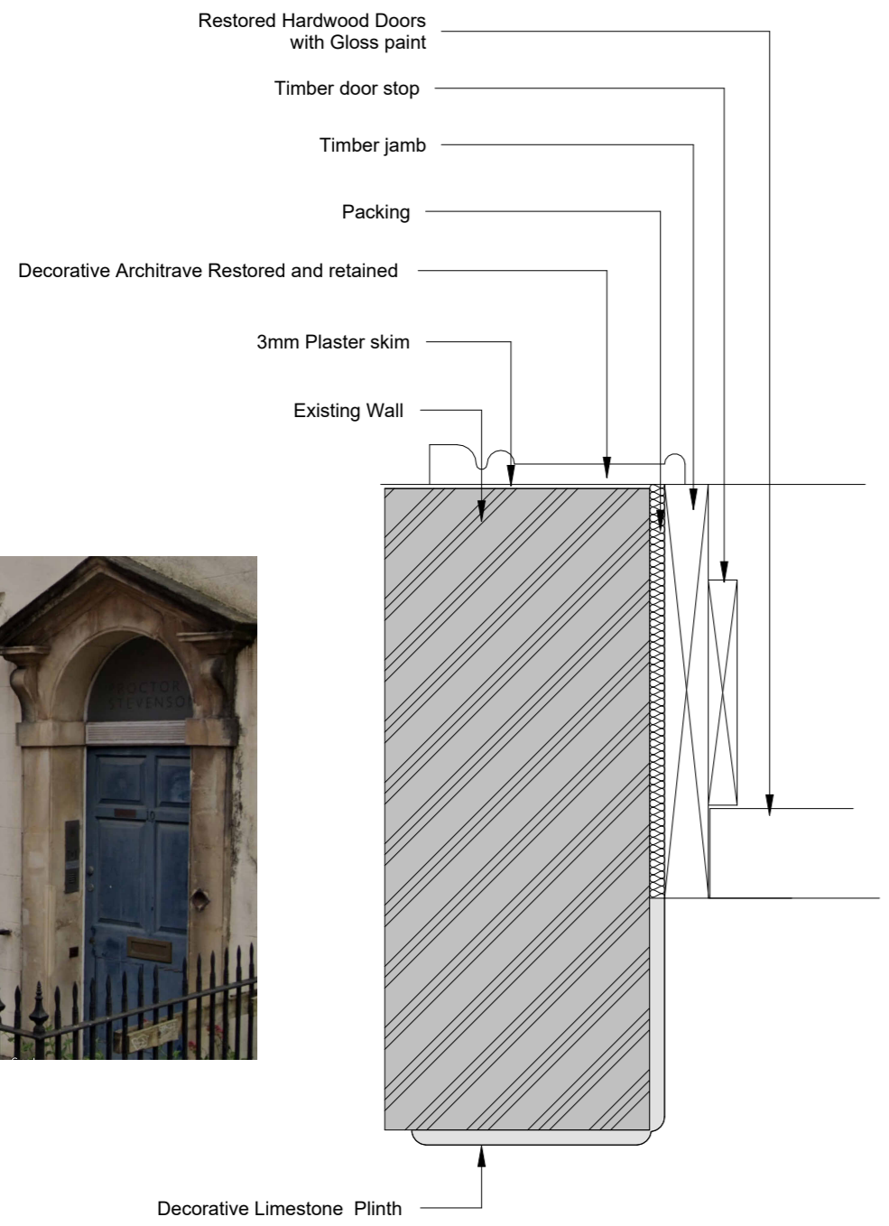
1 Typical External Door Jamb 1 : 5
