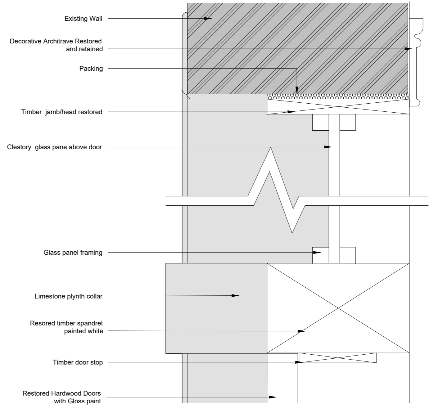
2 Typical External Door head 1 : 5
