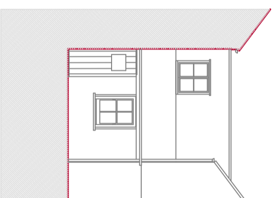
SIDE ELEVATION - As Existing
