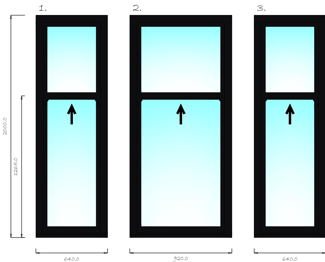
Front Elevation
