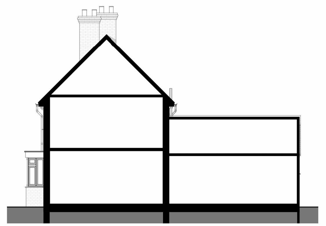
SIDE RIGHT
