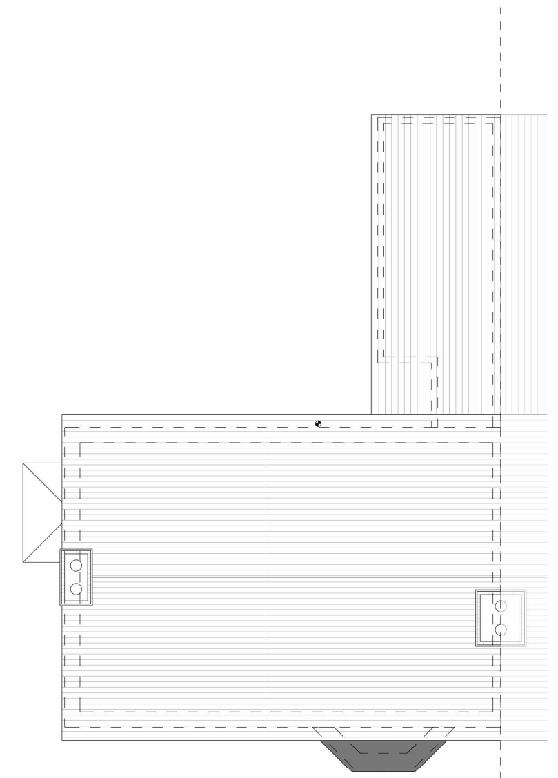
ROOF PLAN
