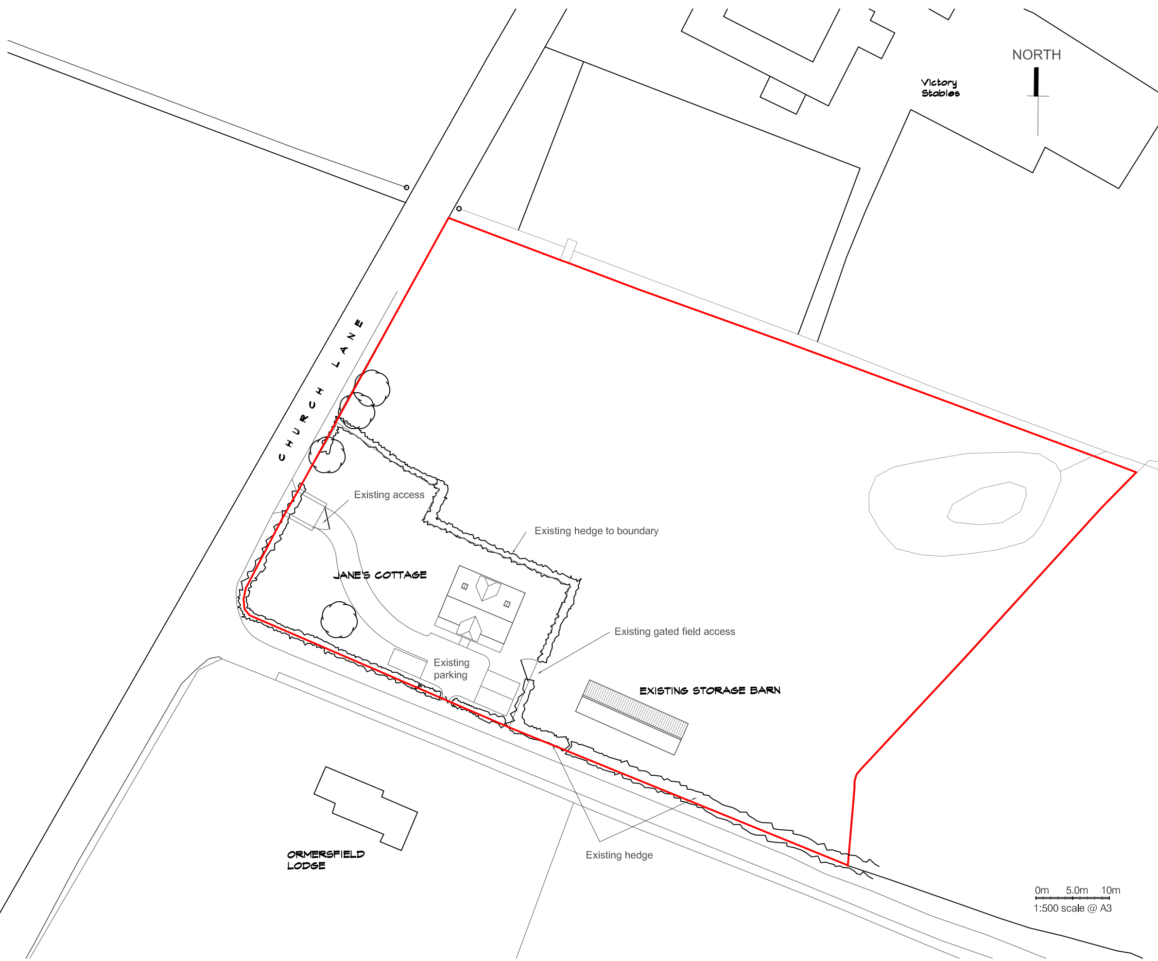
LOCATION PLAN - 1:500
