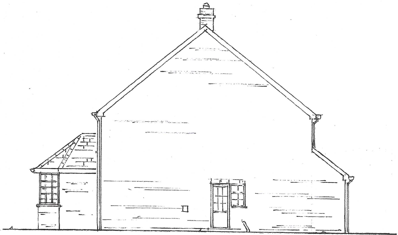
Existing north elevation Scale. 1:100
