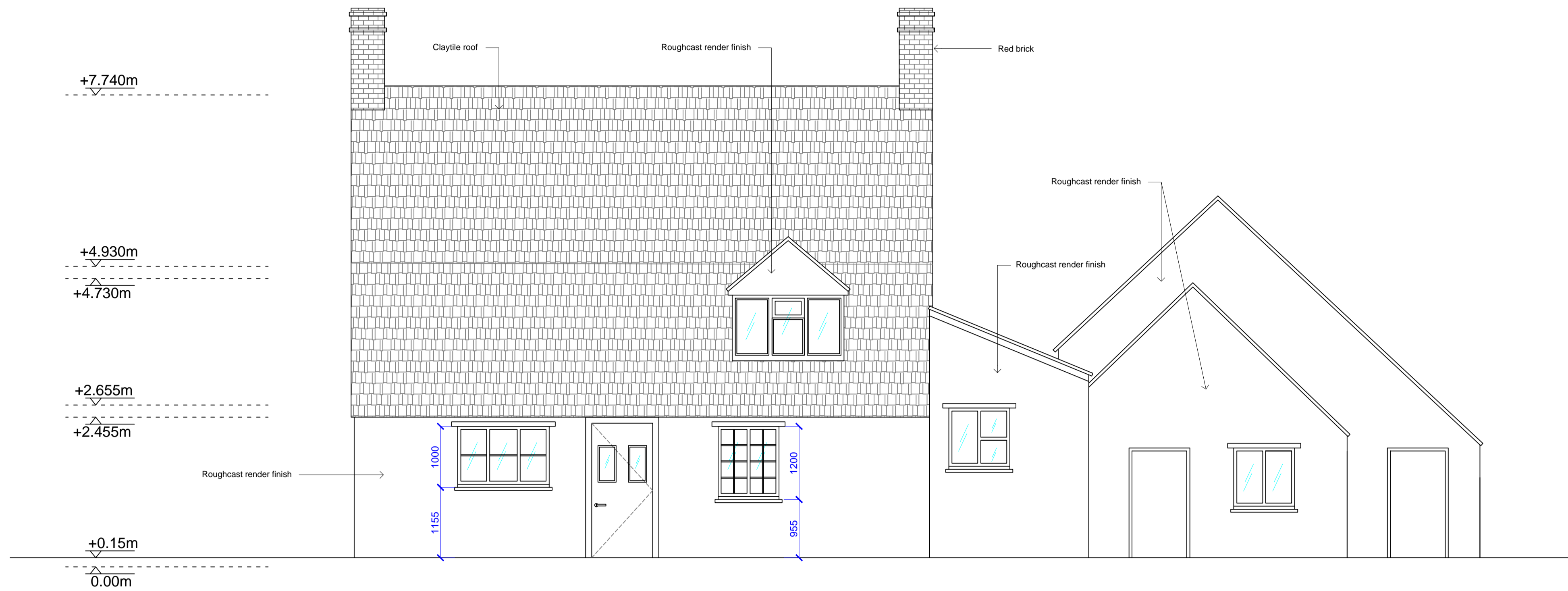
Southeast Elevation
