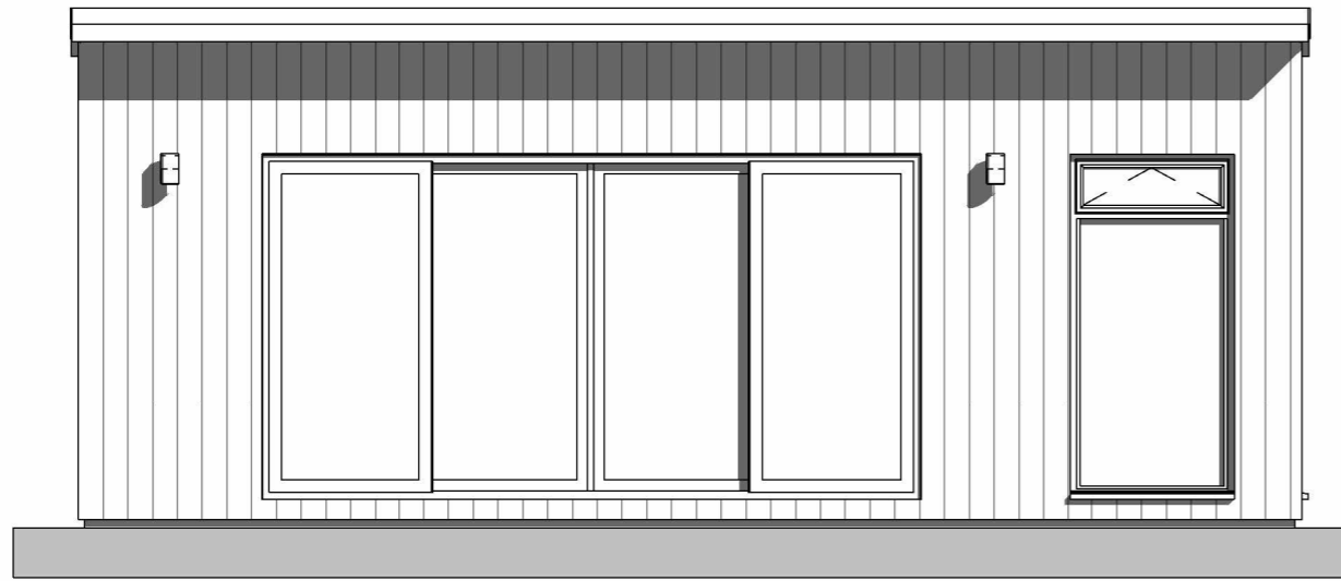
1 Front Elevation 1 : 50
