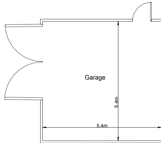
FLOOR PLAN
