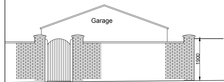
RIGHT SIDE ELEVATION - view from Farriers Way
