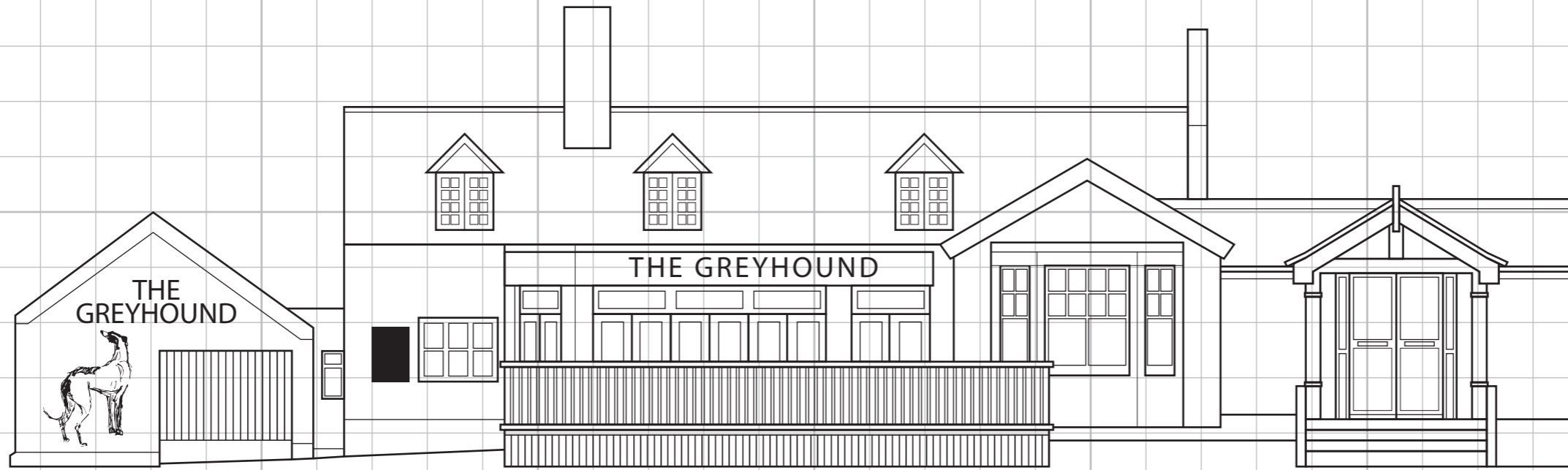
EXISTING ELEVATIONS
