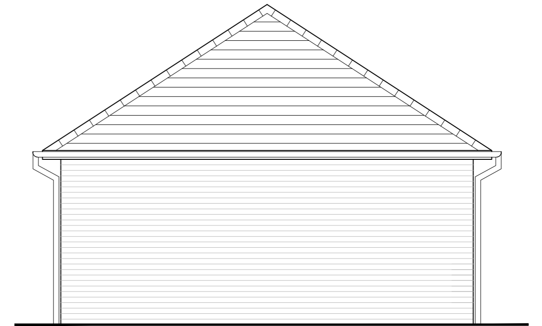
Existing Rear Elevation 1:50 @ A3
