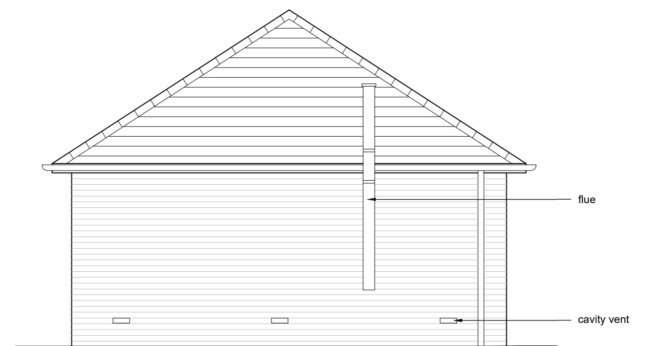
Proposed Side Elevation 1:50 @ A3
