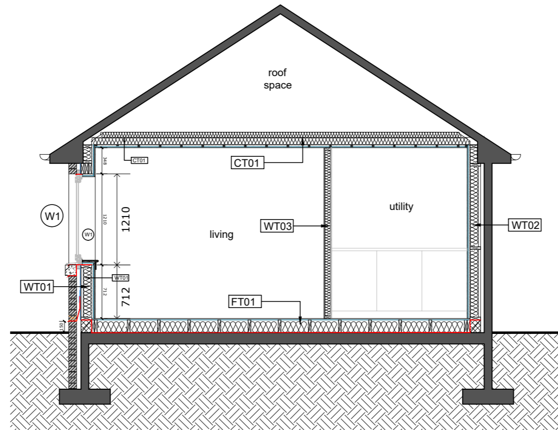
Proposed Section A-A 1:50 @ A3
