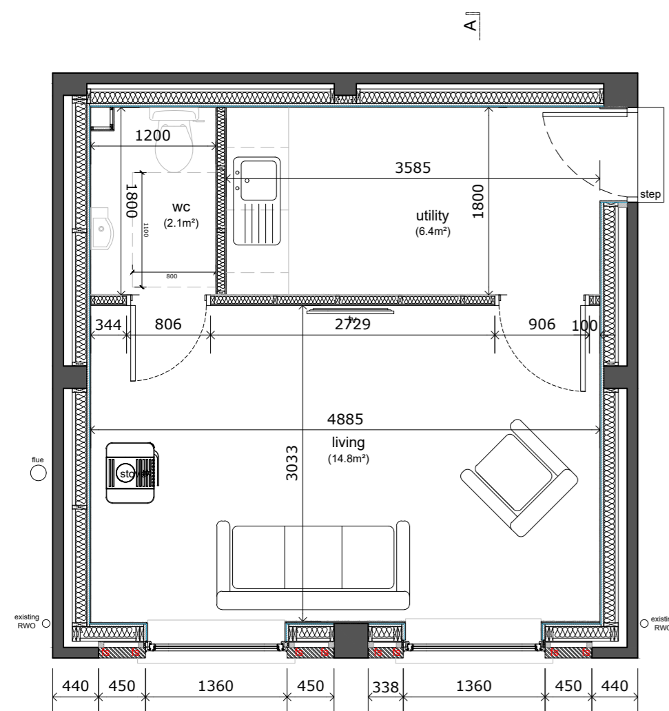
Proposed Floor Plan 1:50 @ A3
