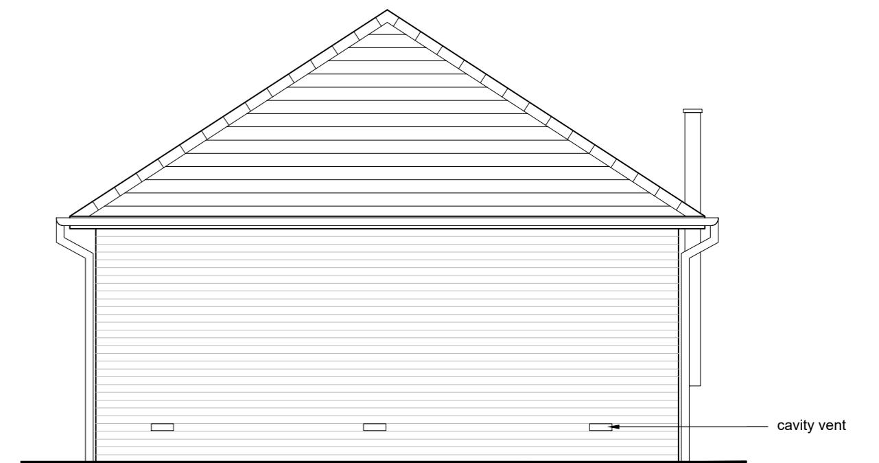
Proposed Rear Elevation 1:50 @ A3
