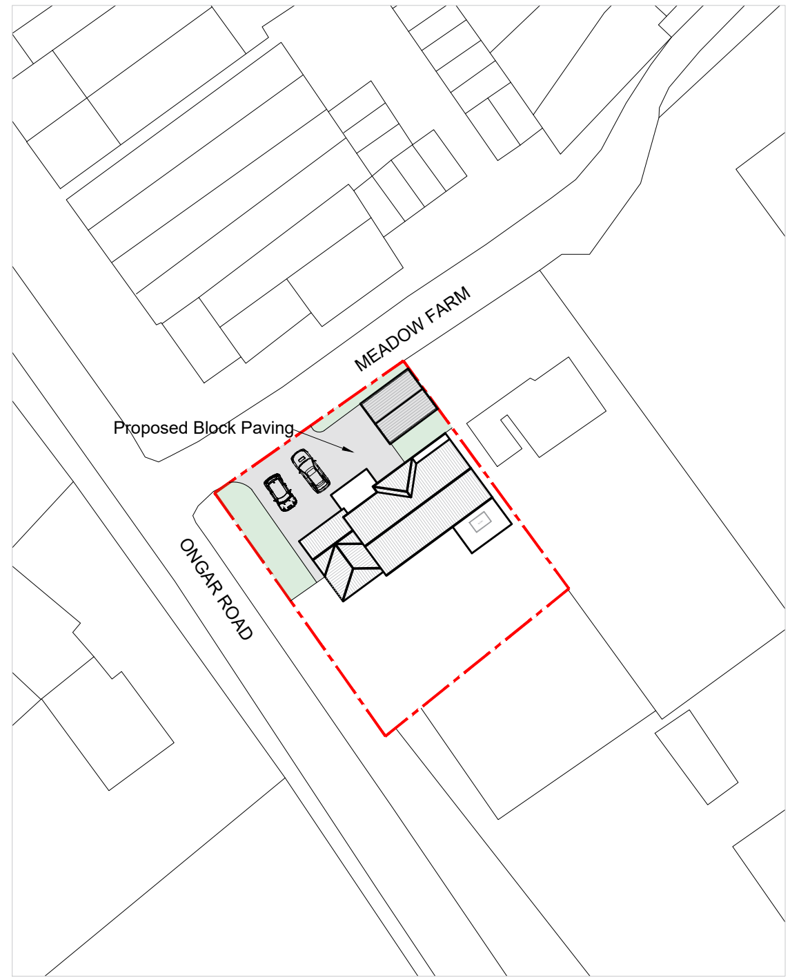
2 Proposed Block Plan 1:500
