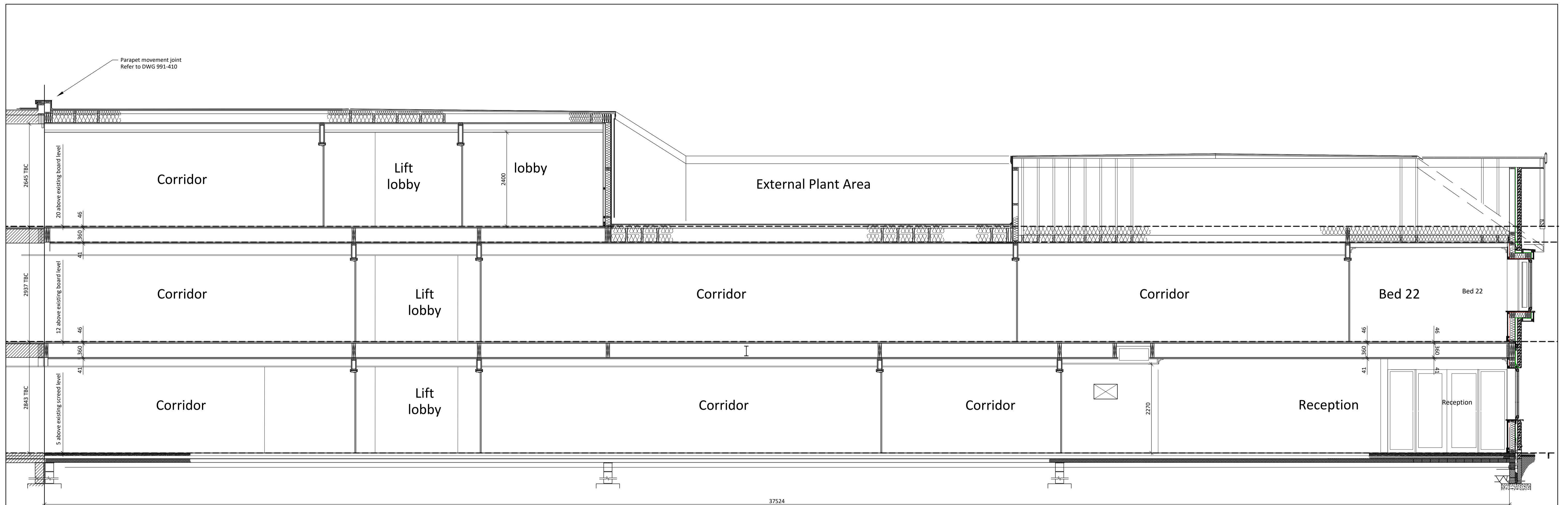
EXISTING PROPOSED BUILDING DIVISION LINE SECTION A-A
