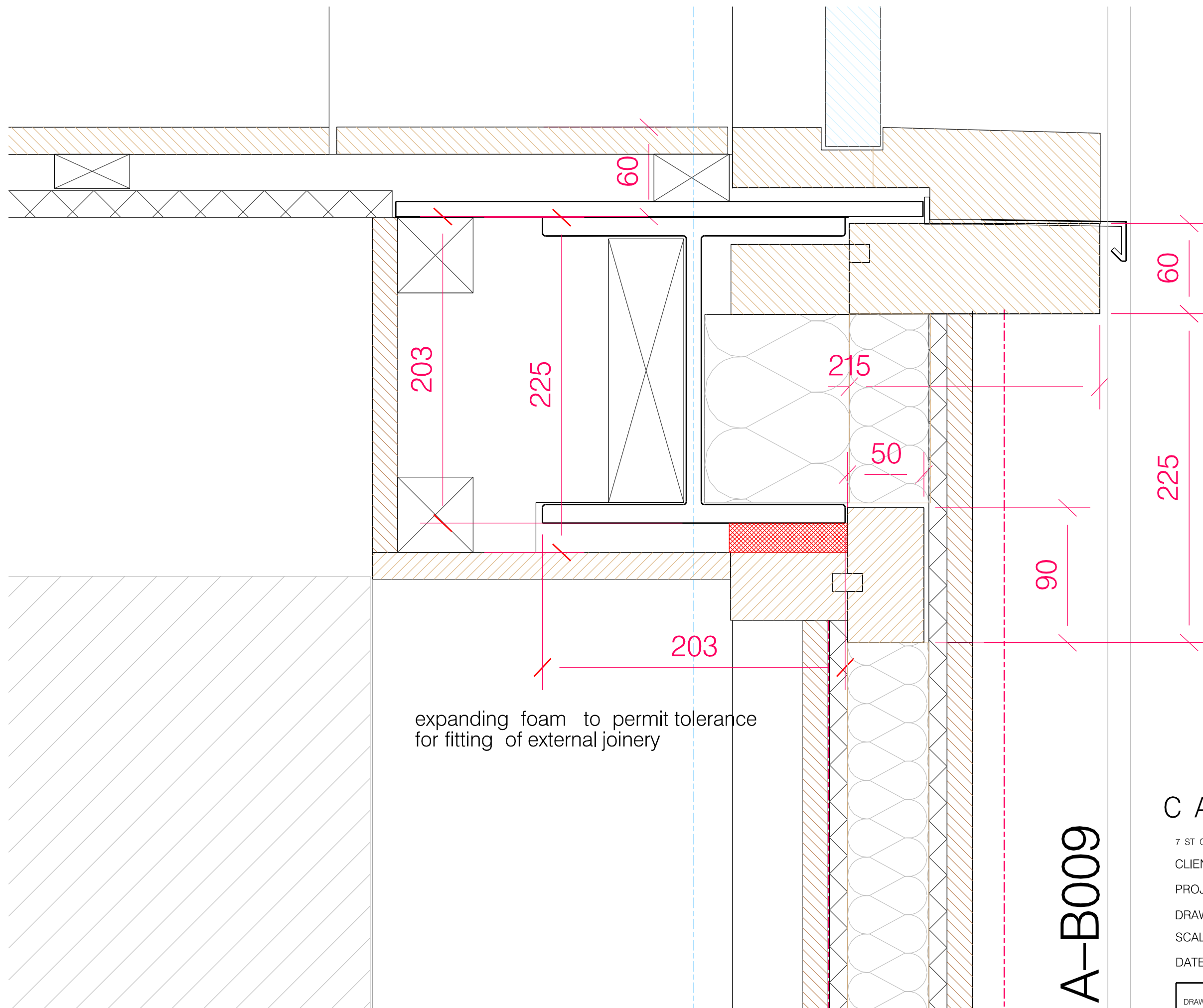
1801 A -B009 section detail showing expanding foam
