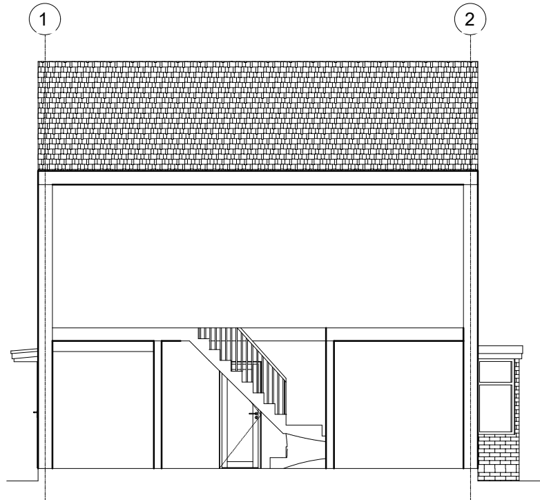
EXISTING SECTION
