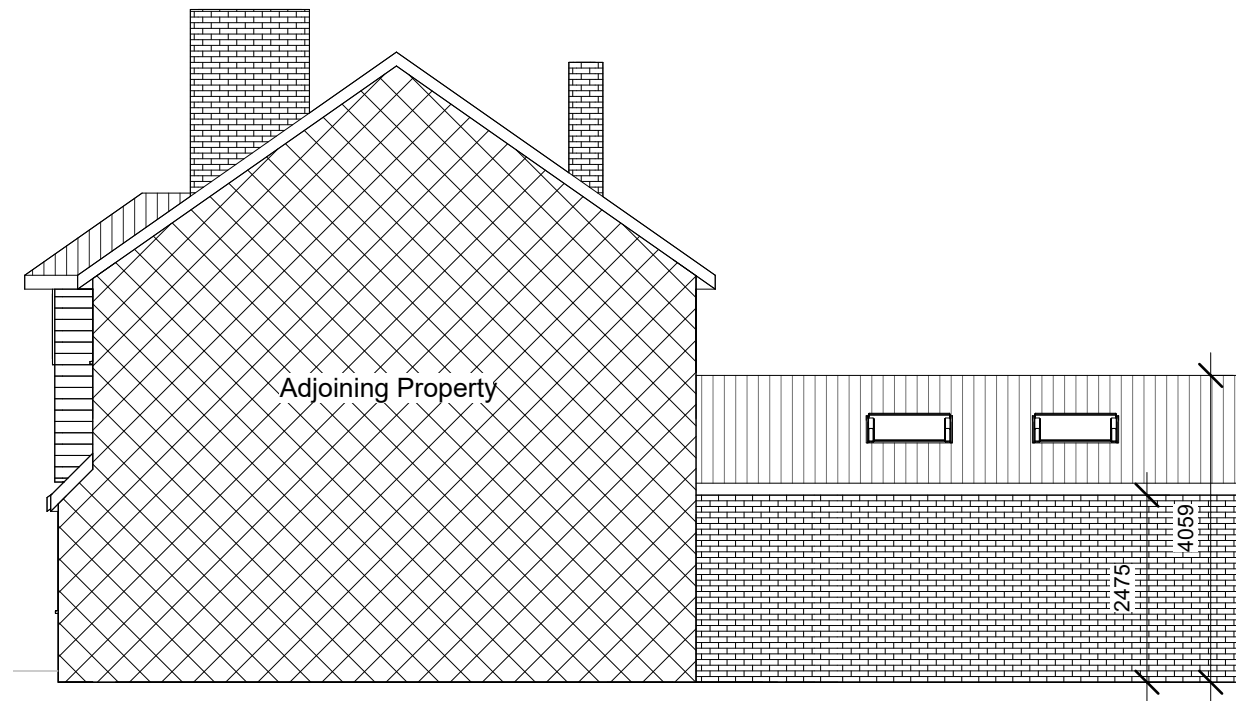
Proposed Side A Elevation
