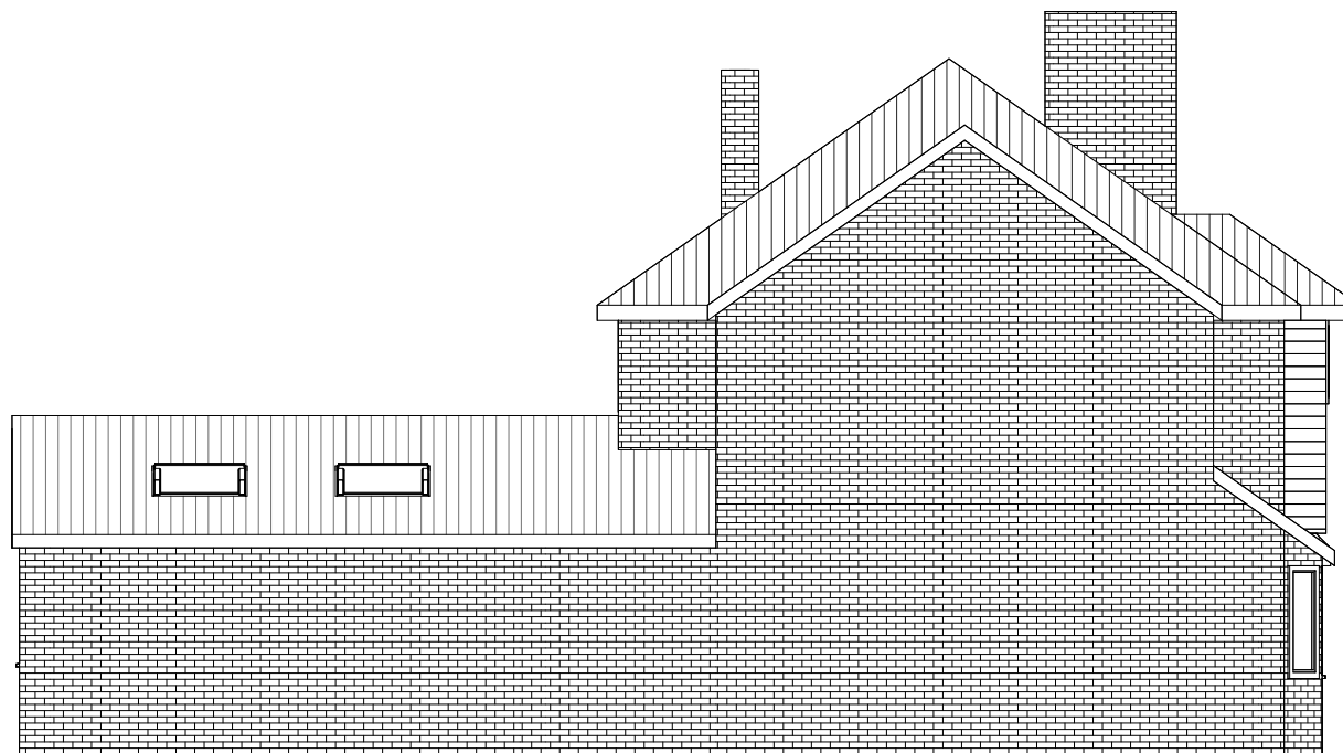
4 Proposed Side B Elevation 1 : 100
