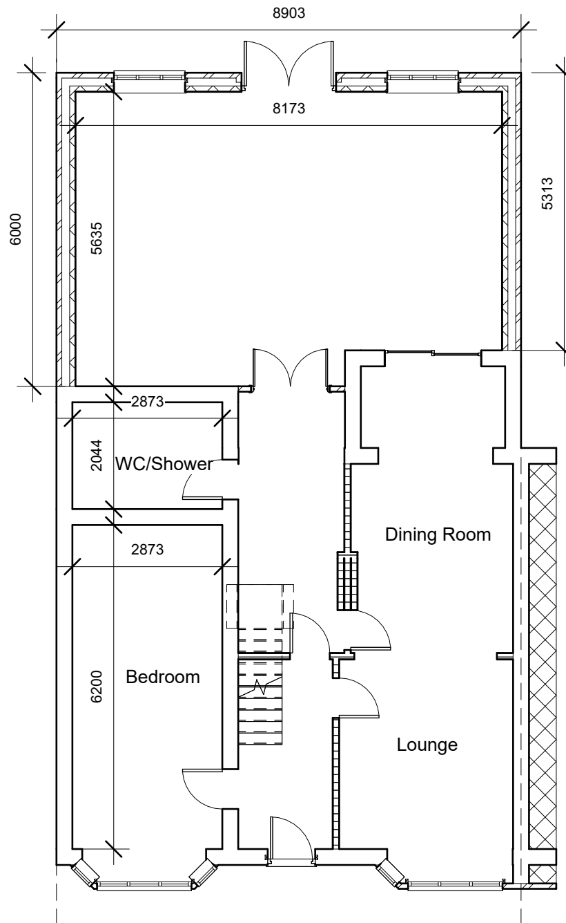
2 Proposed Ground Floor 1 : 100
