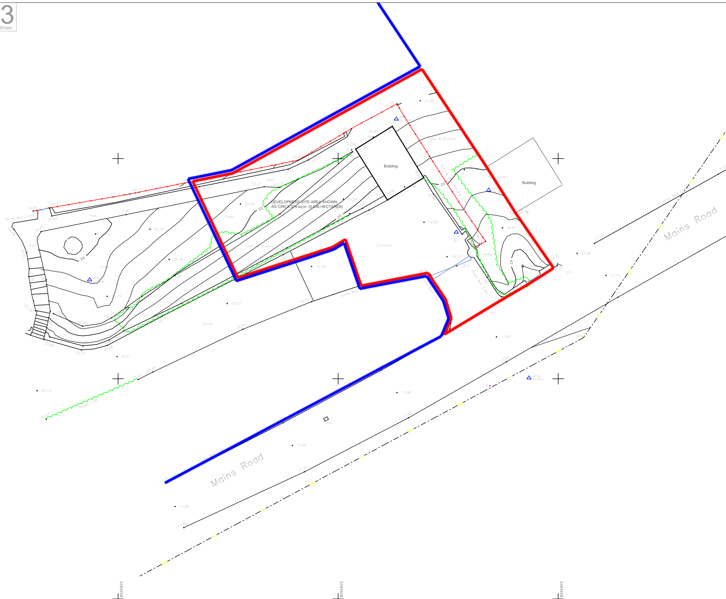
Existing Topographical Plan 1:200
