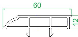
4012 Sash Stop
