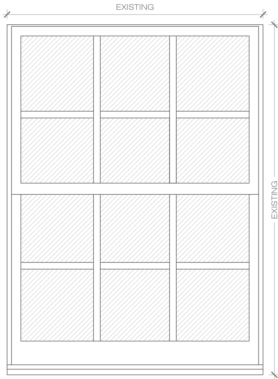
01 Proposed Replacement Double Glazed Window 1:10
