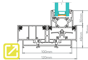
XPSLIDE Panoramic Twin Track
