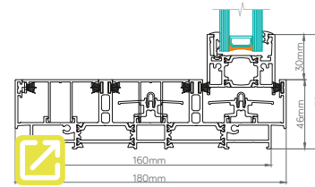
XPSLIDE Panoramic Triple Track
