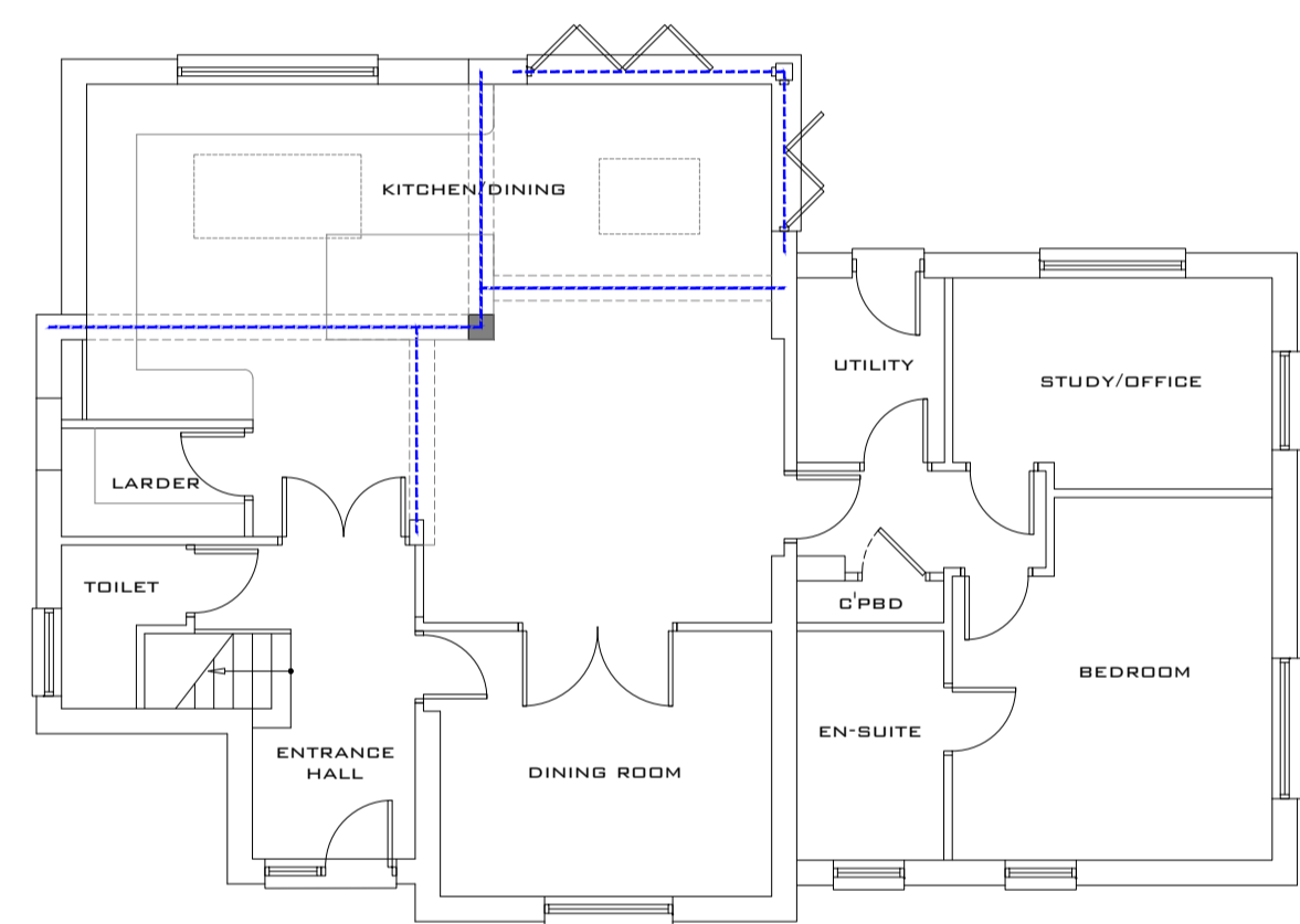
03 PROPOSED GROUND FLOOR PLAN 1:50 @ A1
