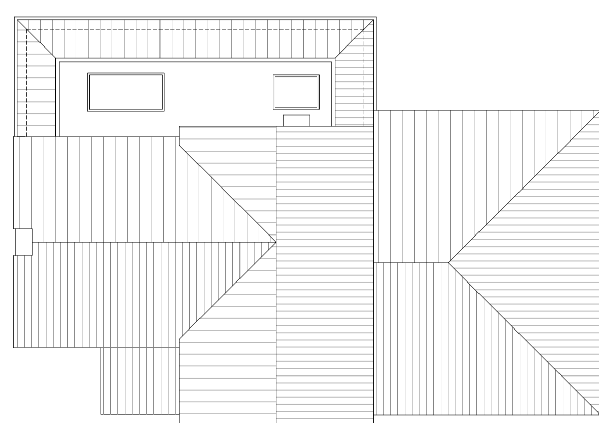
04 PROPOSED ROOF PLAN 1:50 @ A1
