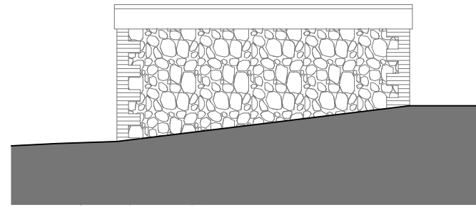
EXISTING GARAGE SIDE (SOUTH EAST FACING) ELEVATION
