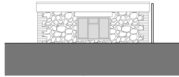
EXISTING GARAGE REAR ELEVATION
