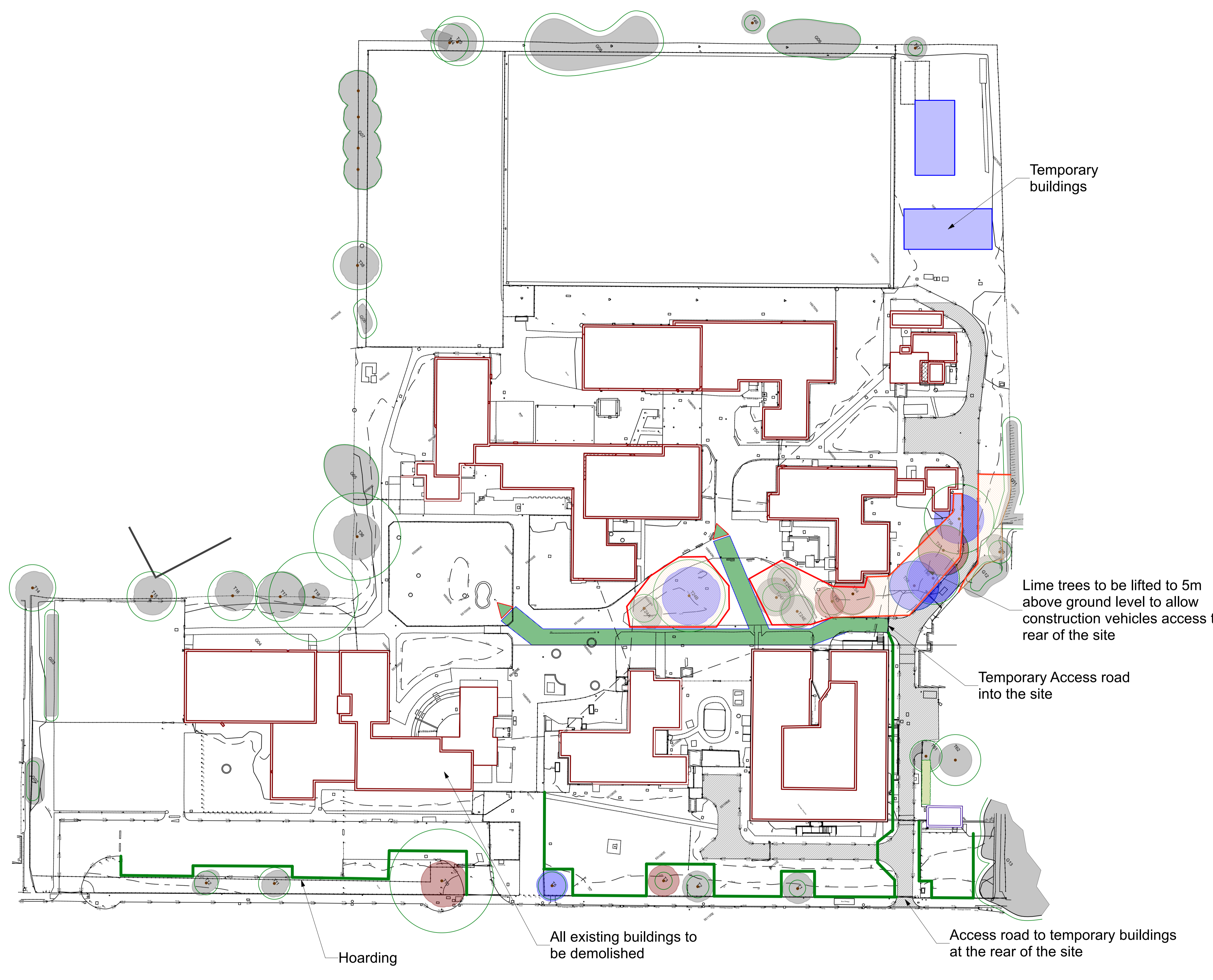
1 Tree Protection Plan Scale: 1:500
