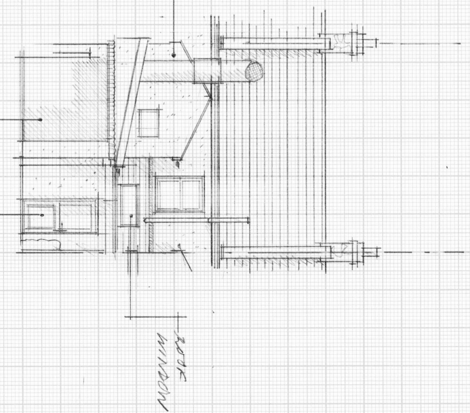
REAR ELEVATION - VIEW FROM NORTH WEST
