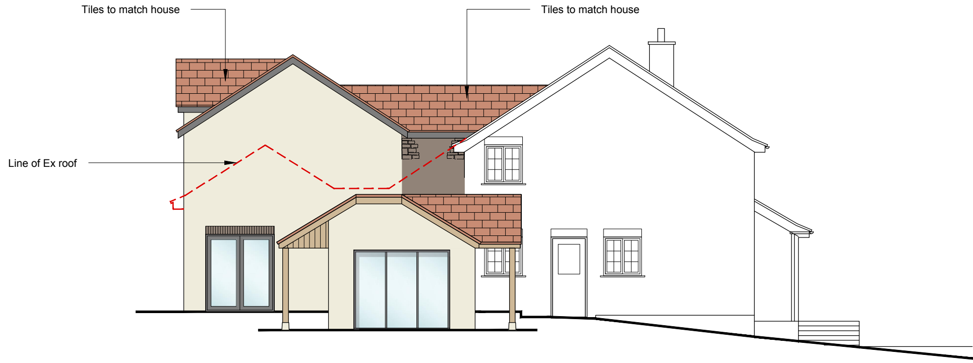
○ East Elevation as Proposed Scale: 1:100
